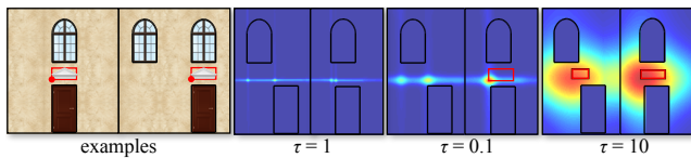
Figure 16: Effects of changing the kernel size: In two examples, a small roof is placed between a door and a window (left). The score for the lower left edge point is shown as heat maps. The upper window is strongly misaligned, the lower window only slightly. With a small \tau as the kernel size, both misalignments are too strong to be considered similar to the examples, while with a big kernel size, both misalignments are considered similar.
