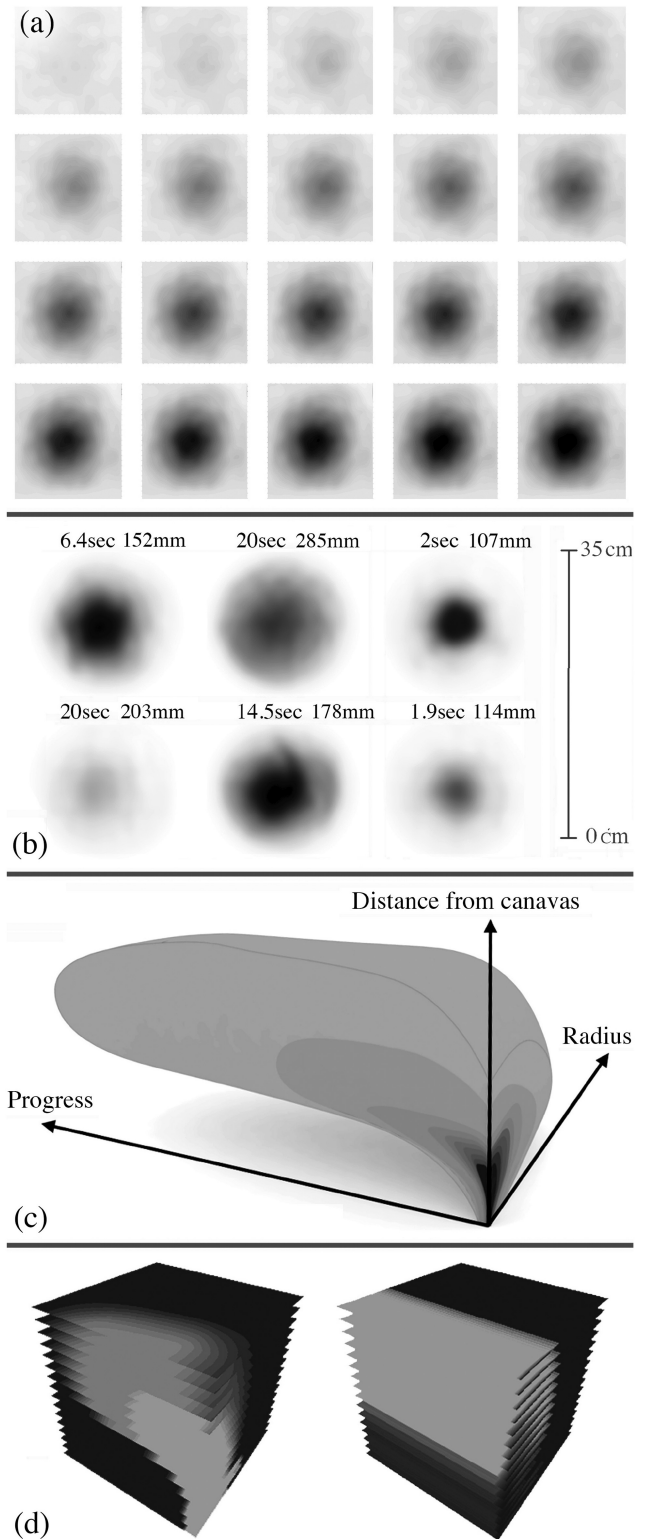
Fig. 4. Spray physical model. (a) Equidistant samples of spray distribution (100msec between samples); (b) aligned spray measurements; (c) illustration of the analog SDIF; (d) the sampled SDIF and ITSF as represented in the GPU as 3D textures.
